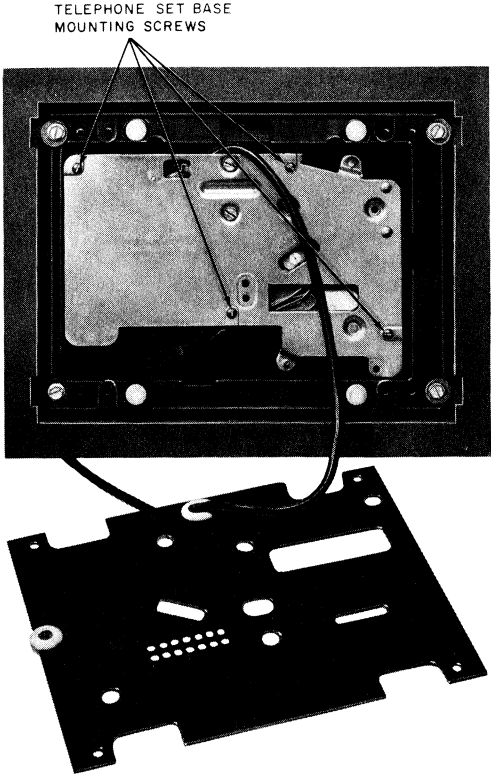
Fig. 7—Removing Telephone Set Base
